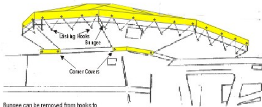
Bungee can be removed from hooks to flip open as much hopper as desired.
